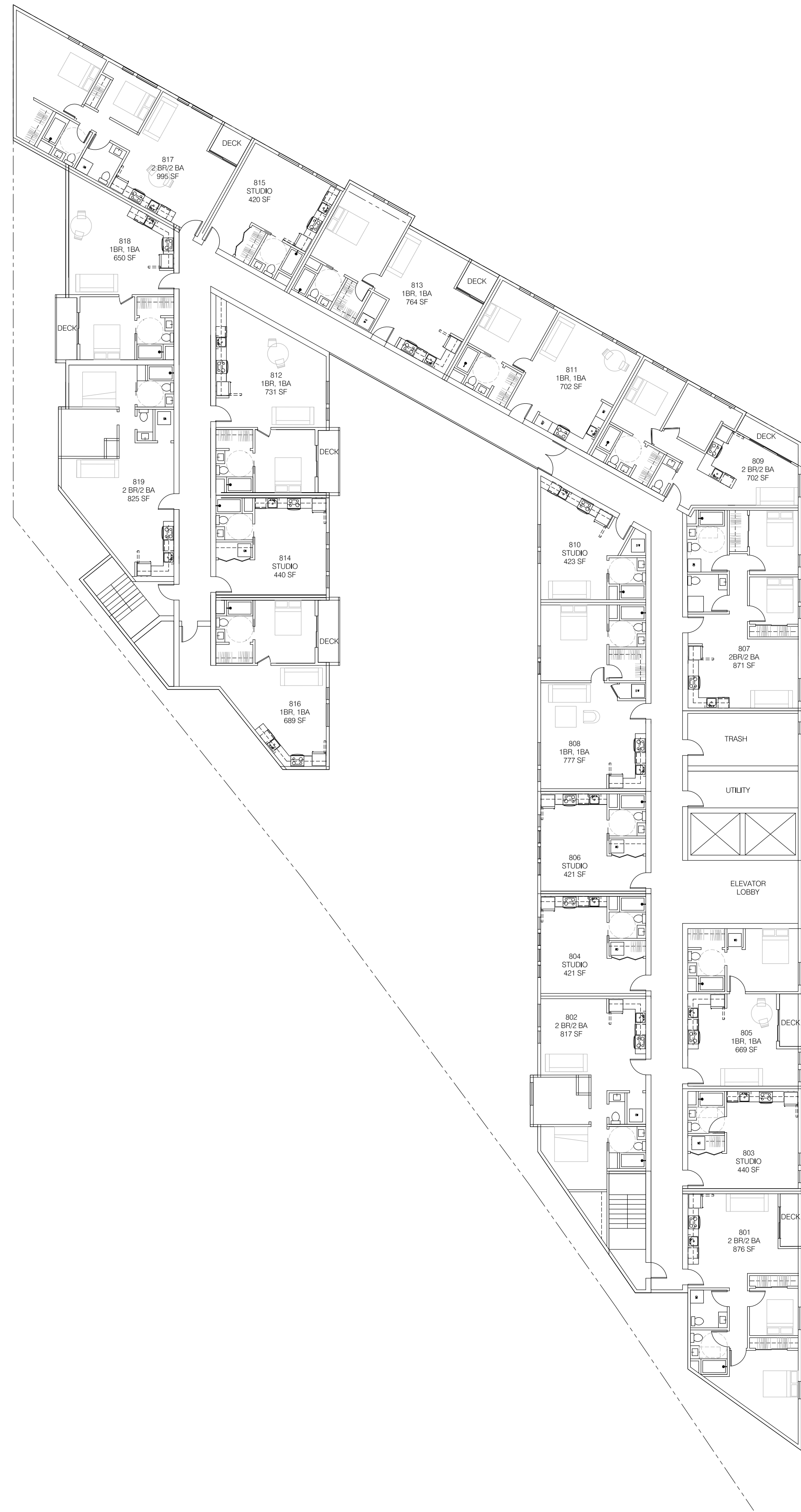
2 8TH FLOOR PLAN 1/16" = 1'-0"
