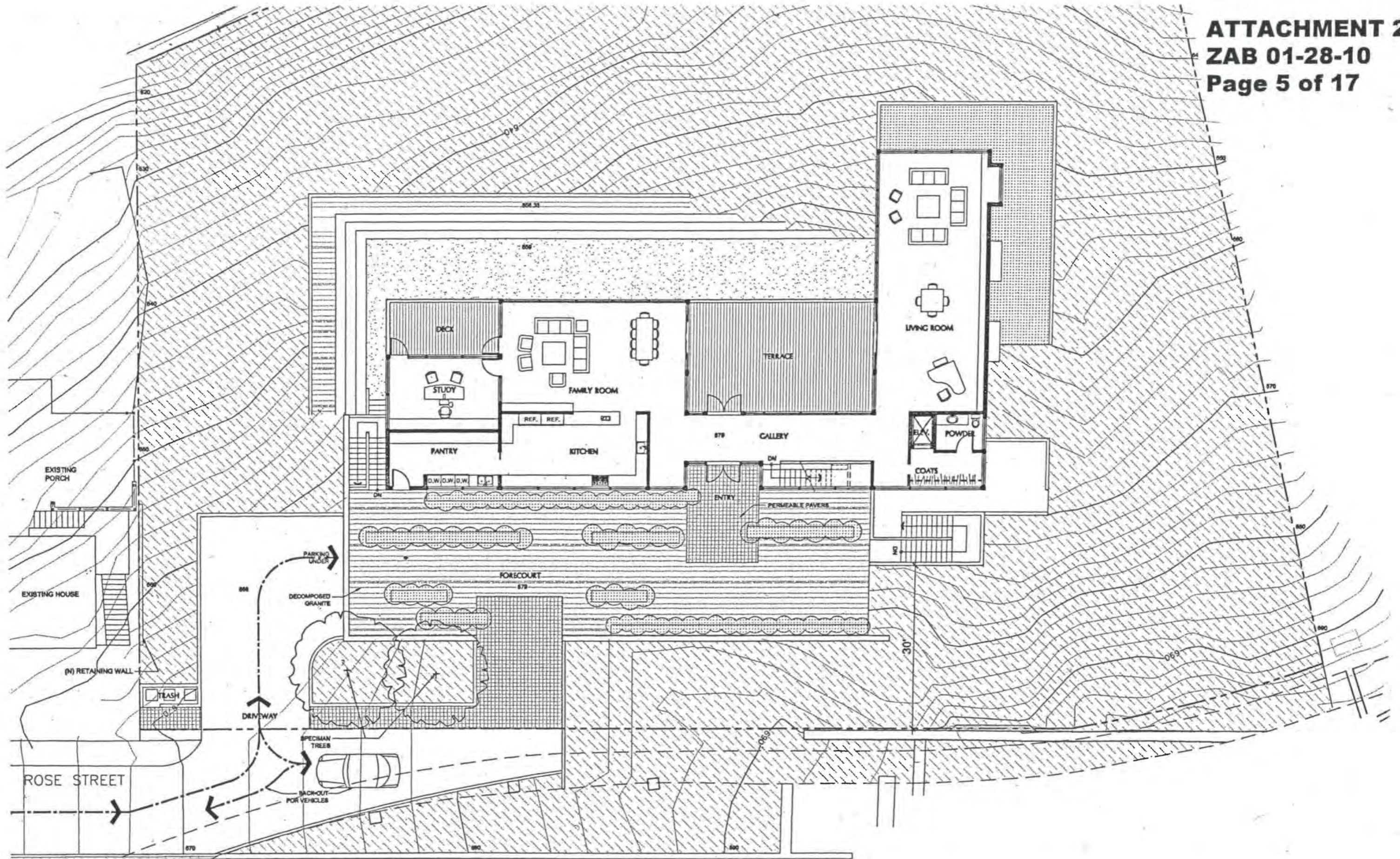
UPPER FLOOR PLAN WITH REVISED DRIVEWAY
