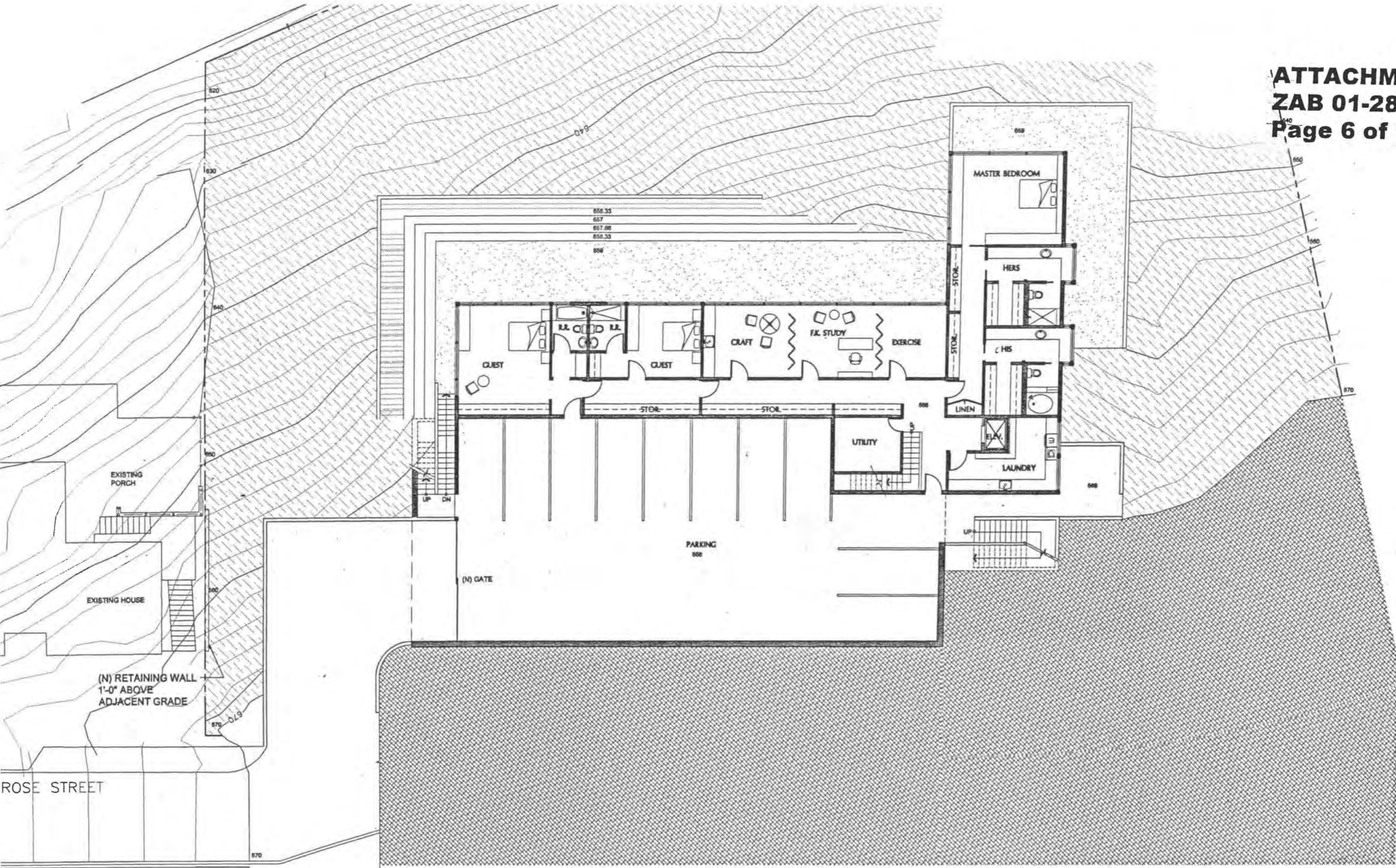
LOWER FLOOR PLAN WITH REVISED DRIVEWAY
