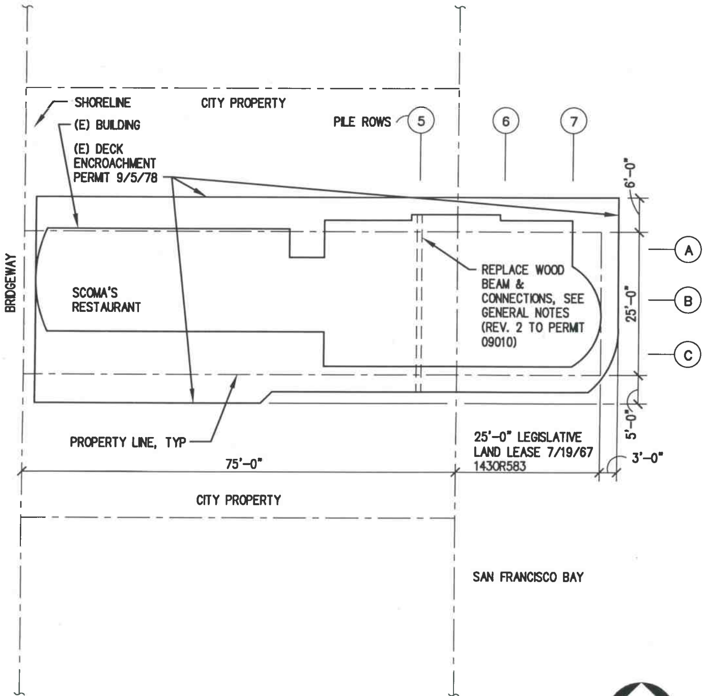
1 SITE & BUILDING PLAN A1 588 BRIDGEWAY, SAUSALITO
