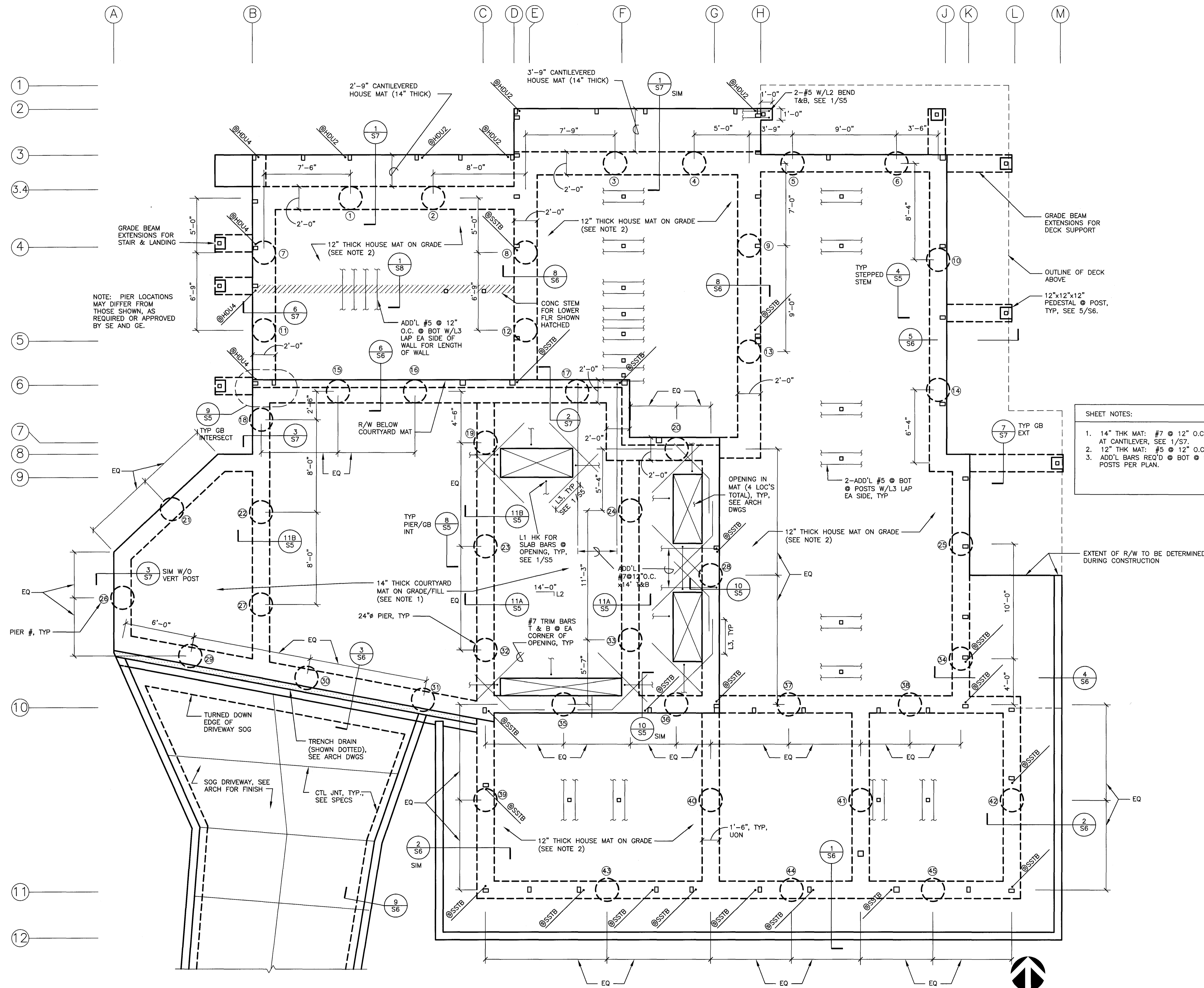
1 FOUNDATION PLAN
